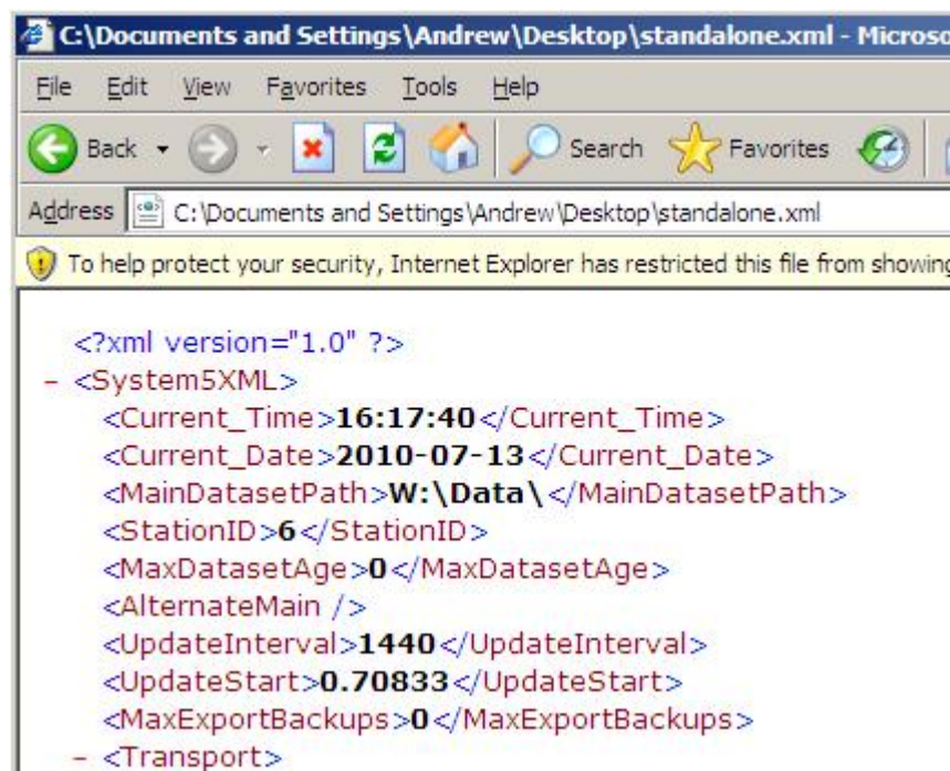
Figure 1 - standalone.xml file before version 6 path updates.
