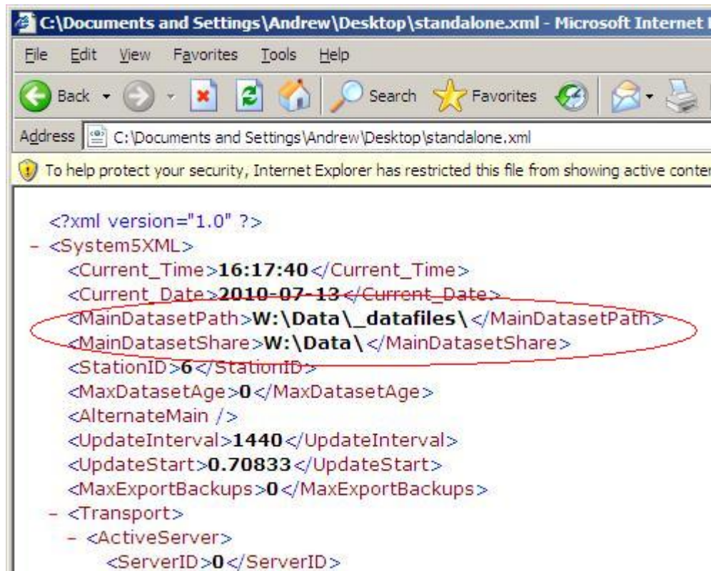
Figure 2 - standalone.xml after the version 6 changes.
